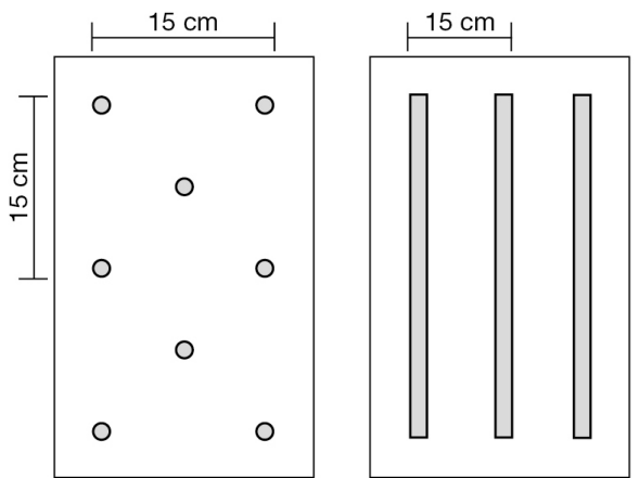
Spot-bonding technique
