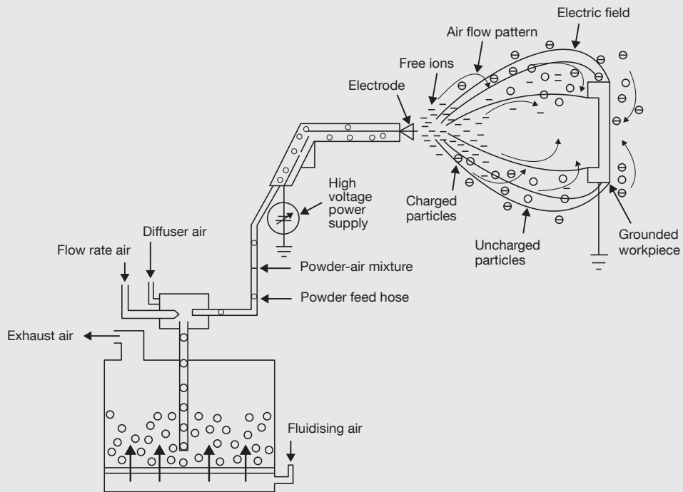
Image 7.7 High voltage powder sprayer.
